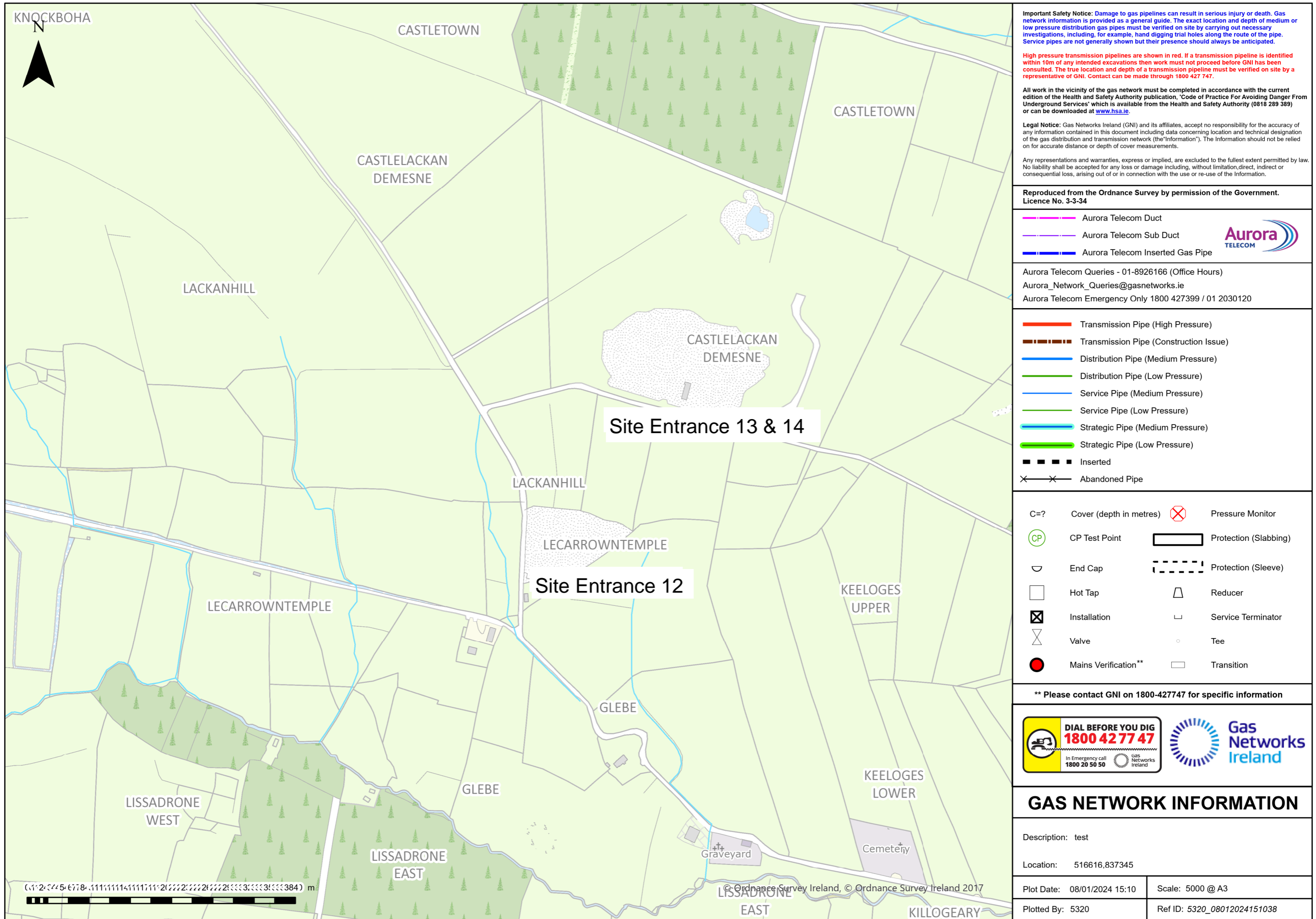
Figure 13.8 - Gas Network Information at Site Entrances 12, 13 & 14
